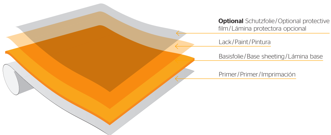
Einschicht- (Uni-)Folie / Single-layer (plain color) film / Lámina monocapa (uniforme)
